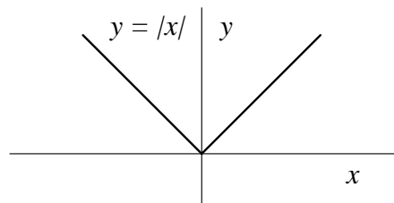
The Graph of y = |x| .
